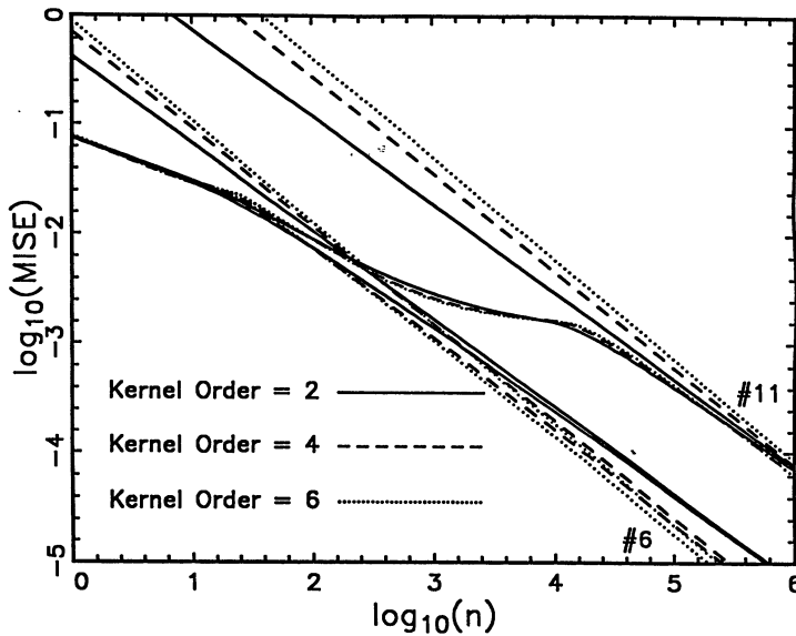
FIG. 9. \log_{10}(\inf_{h>0} \text{MISE}(h)) and \log_{10}(\inf_{h>0} \text{AMISE}(h)) as a function of \log_{10}(n) for the bimodal density, #6, and the double claw density, #11, and Gaussian-based kernel orders p = 2 (solid), 4 (dashed), 6 (dotted). The AMISE's are represented by straight lines. The corresponding MISE's are curves that are always below, but asymptotic to, the AMISE's. All density #11 curves are above the corresponding density #6 curves.
