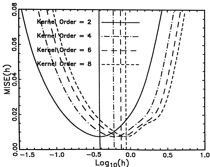
FIG. 8. MISE(h) for the bimodal density, #6, n = 100 , Gaussian based kernels of orders p = 2, 4, 6 and 8 .
